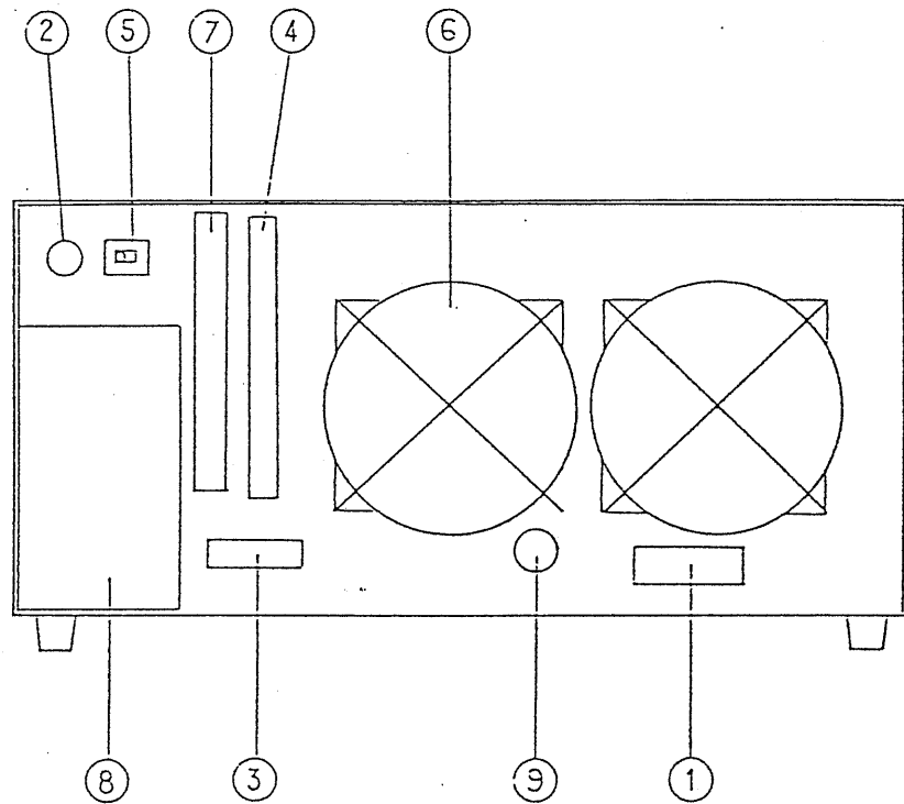
FIG. 2-3 Rear Panel
