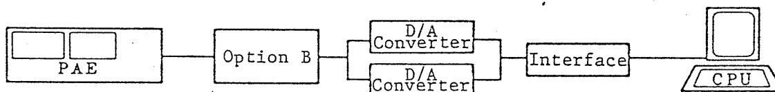
FIG. 2 To control both boltage and current (GP-IB only)
