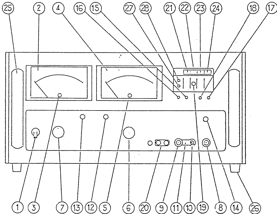
FIG. 2-2 Front Panel
